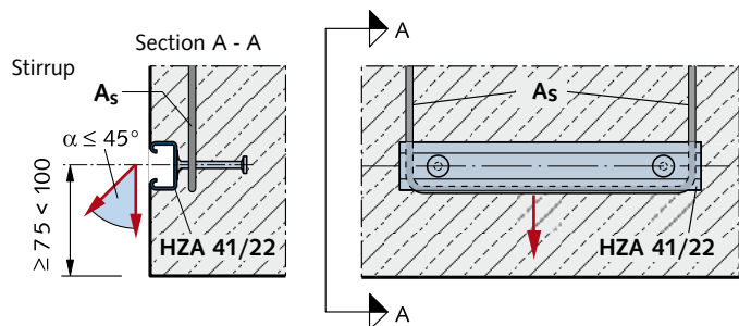
Figure 2: Additional reinforcement placement
