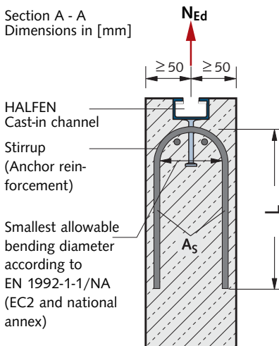
Figure 1: additional reinforcement
