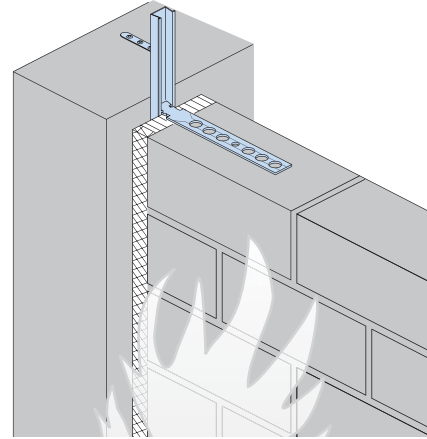
Connection of a load bearing masonry wall as a fire wall according to DIN 4102-4 section 9.8.4 (figure 9.13) or according to DIN EN 1996-1-2: 2011-04 (figure E.4B)
