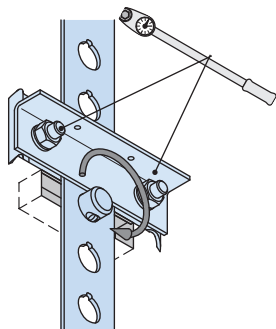
Recommended torque for façade panel cast-in parts
